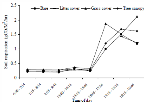
Fig. 2 Effect of time of day on soil respiration.
