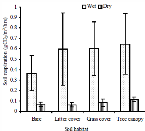
Fig. 1 Soil respiration in the different habitats in the wet and dry seasons.
