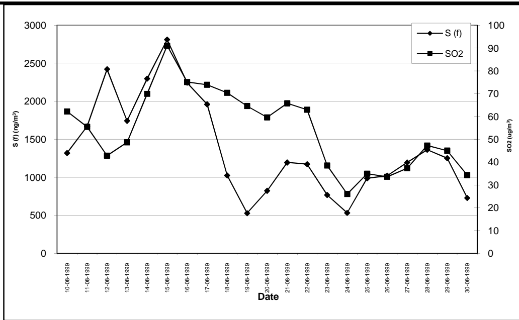
Fig. 2: Time series of S(f) and SO 2
