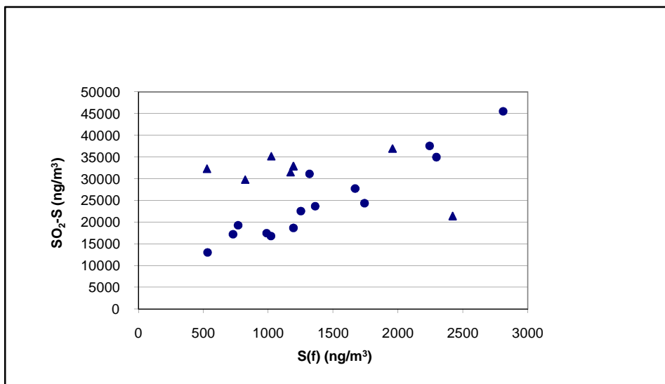
Fig. 3: Regression diagram of SO 2 -S versus S(f) for Gaborone 1999. The regression line refers to the cases of long distance transport (plotted as dots). The equation of the regression line is: y = 13.5x + 5960 \text{ ng/m}^3 . The regression coefficient is R^2 = 0.88 .
