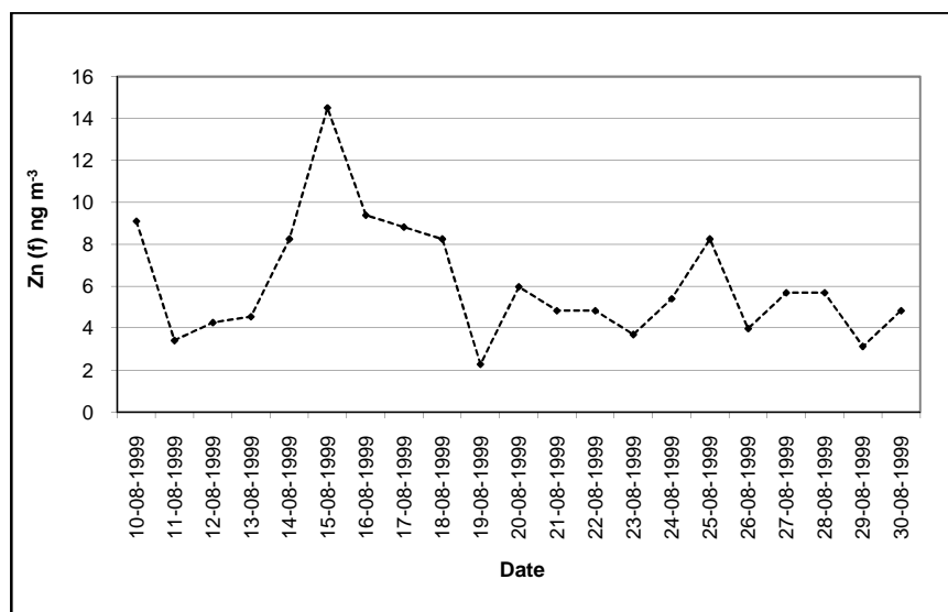
Fig.1: Time series of Zn (f). Zn is mostly found in the fine particle mode and hence it's most probably anthropogenically generated.
